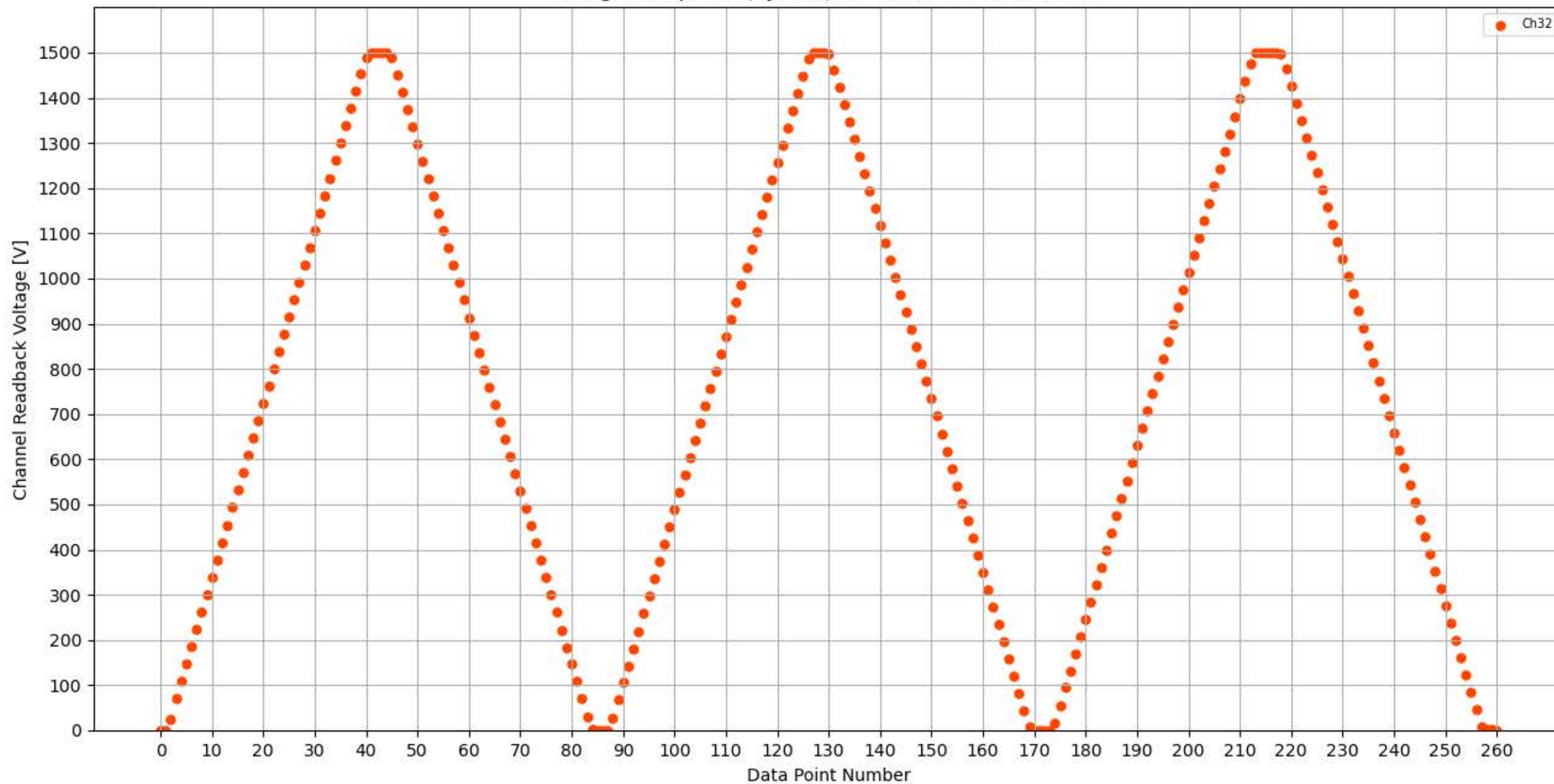
Voltage Ramp Test (Python) Bd #326, Slot #6, Ch #32
