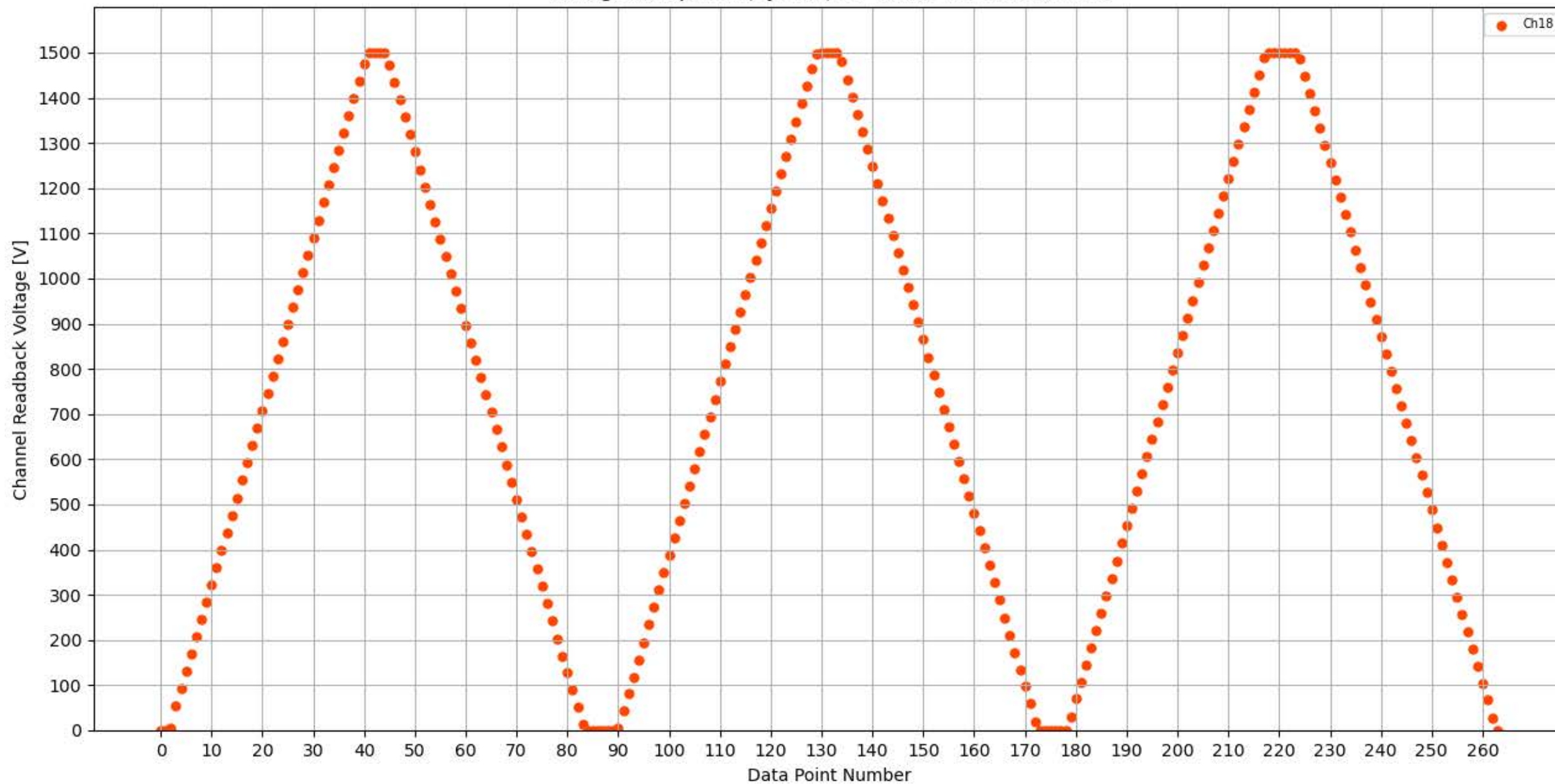
Voltage Ramp Test (Python) Bd #326, Slot #6, Ch #18
