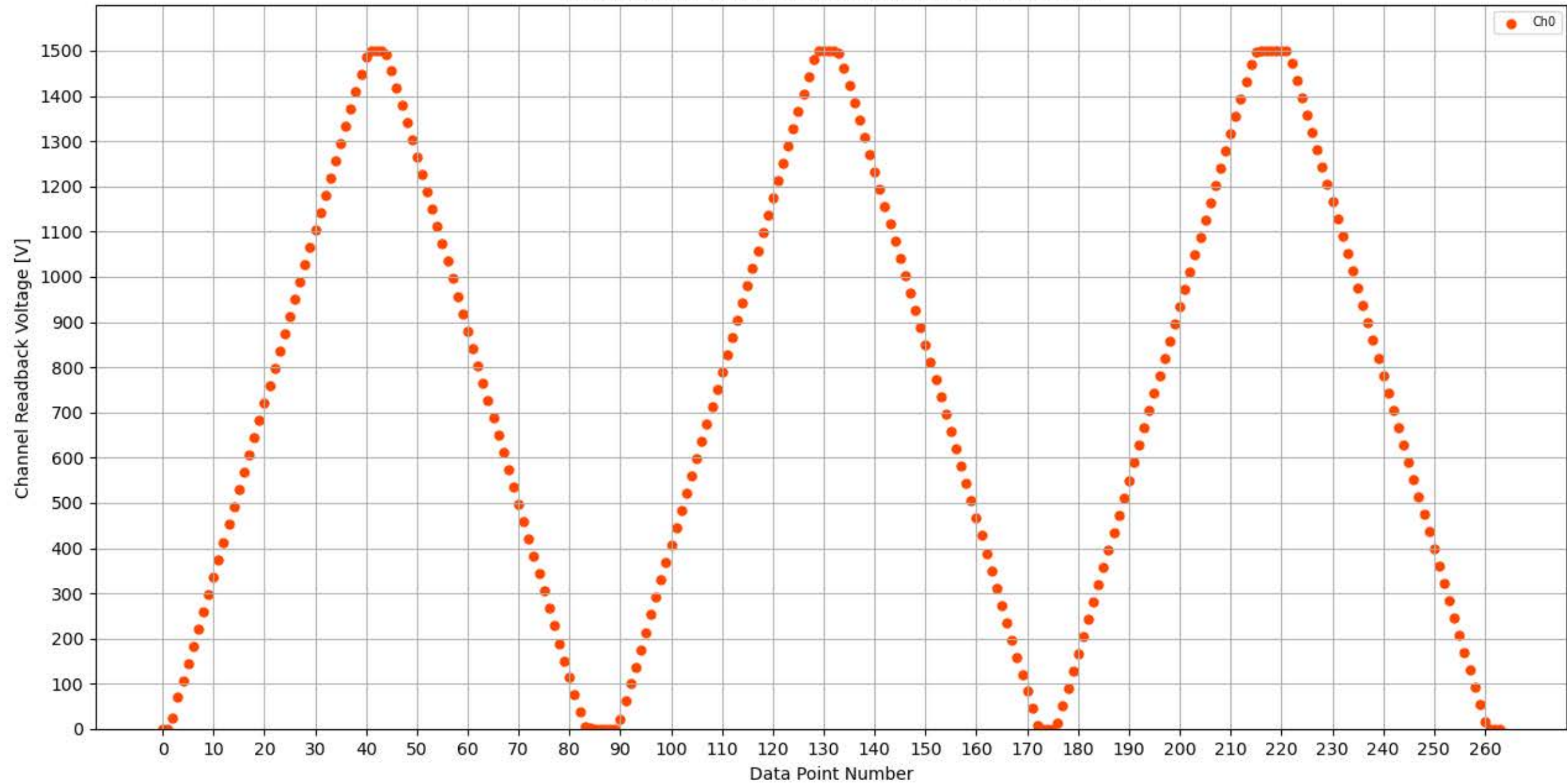
Voltage Ramp Test (Python) Bd #326, Slot #6, Ch #0
