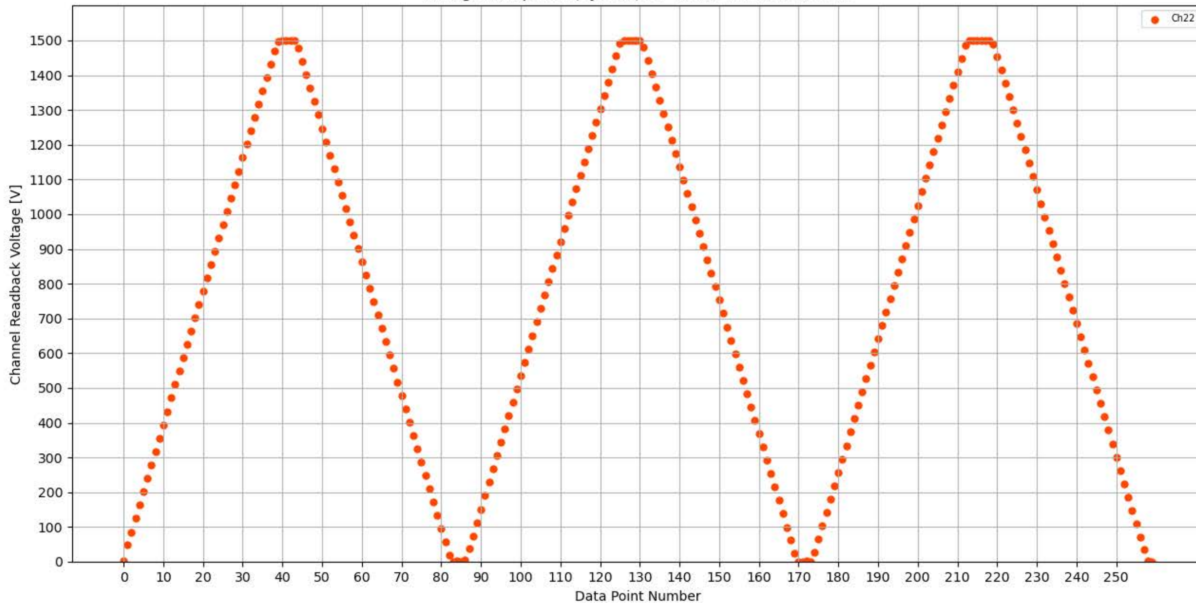
Voltage Ramp Test (Python) Bd #326, Slot #6, Ch #22
