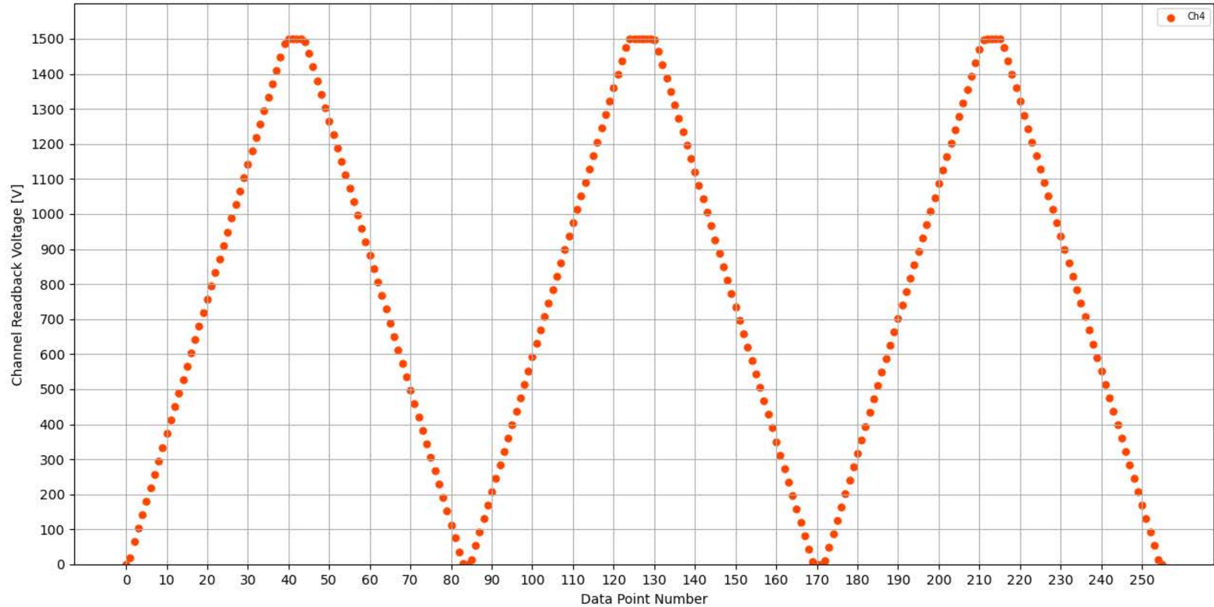
Voltage Ramp Test (Python) Bd #326, Slot #6, Ch #4
