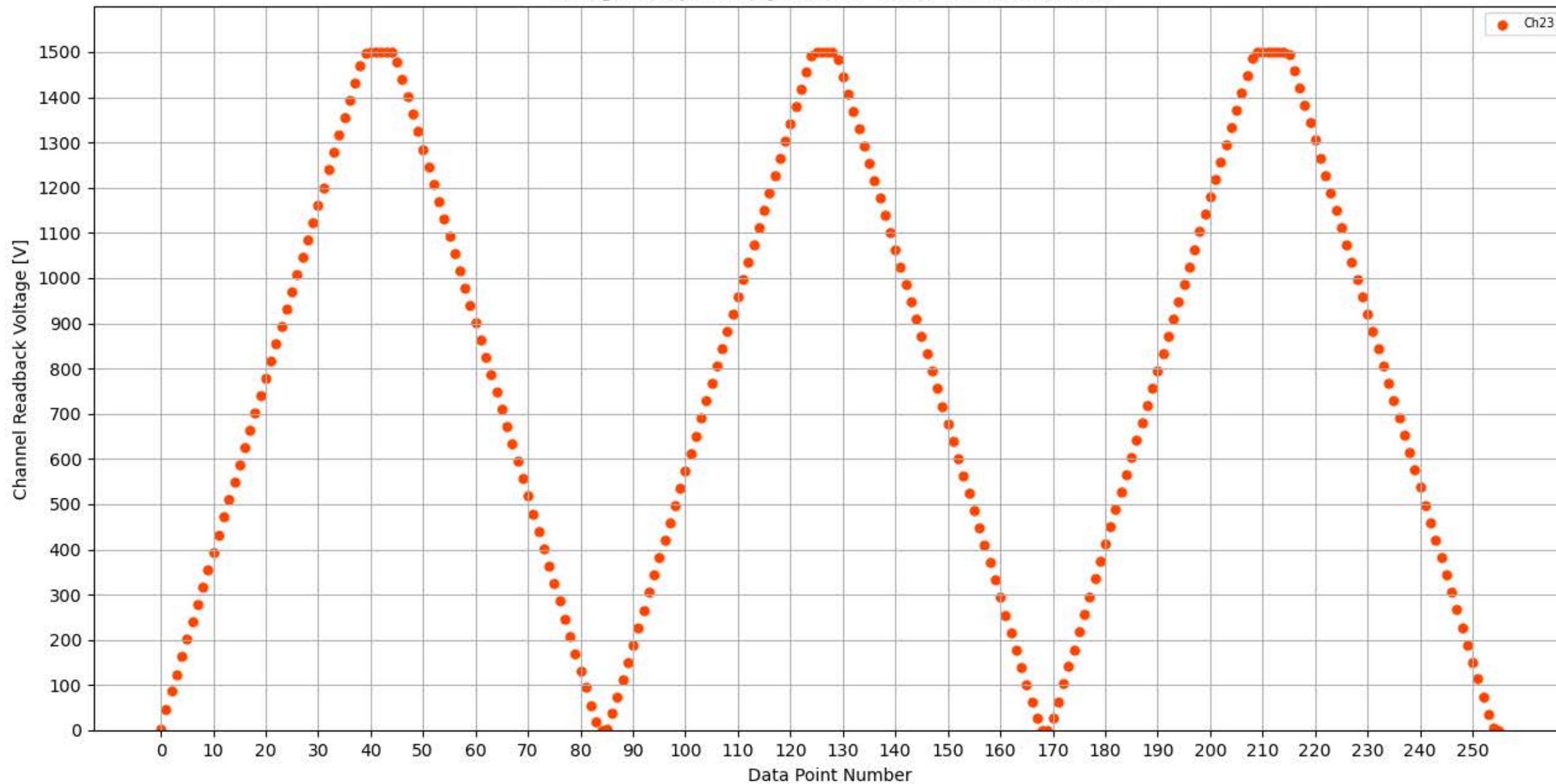
Voltage Ramp Test (Python) Bd #326, Slot #6, Ch #23
