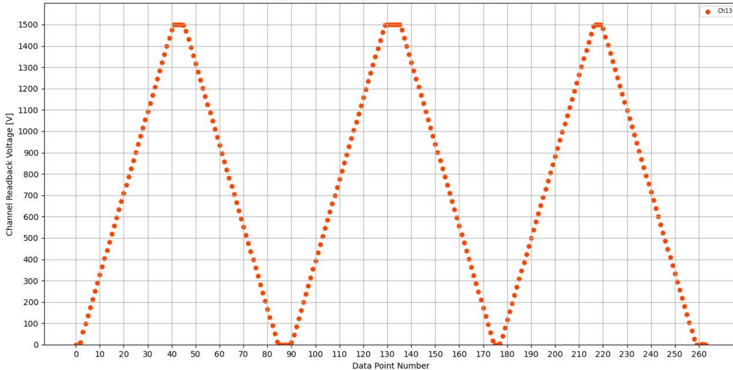
Voltage Ramp Test (Python) Bd #326, Slot #6, Ch #13
