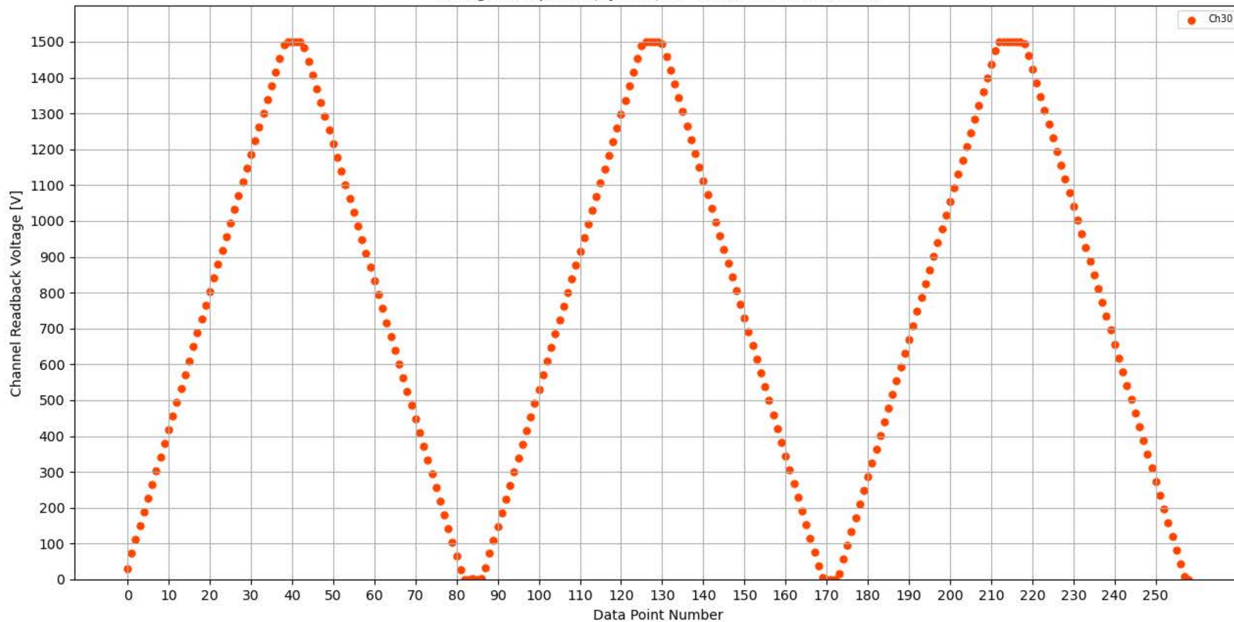
Voltage Ramp Test (Python) Bd #326, Slot #6, Ch #30
