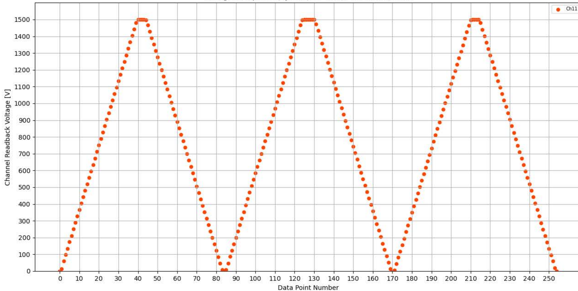
Voltage Ramp Test (Python) Bd #326, Slot #6, Ch #11
