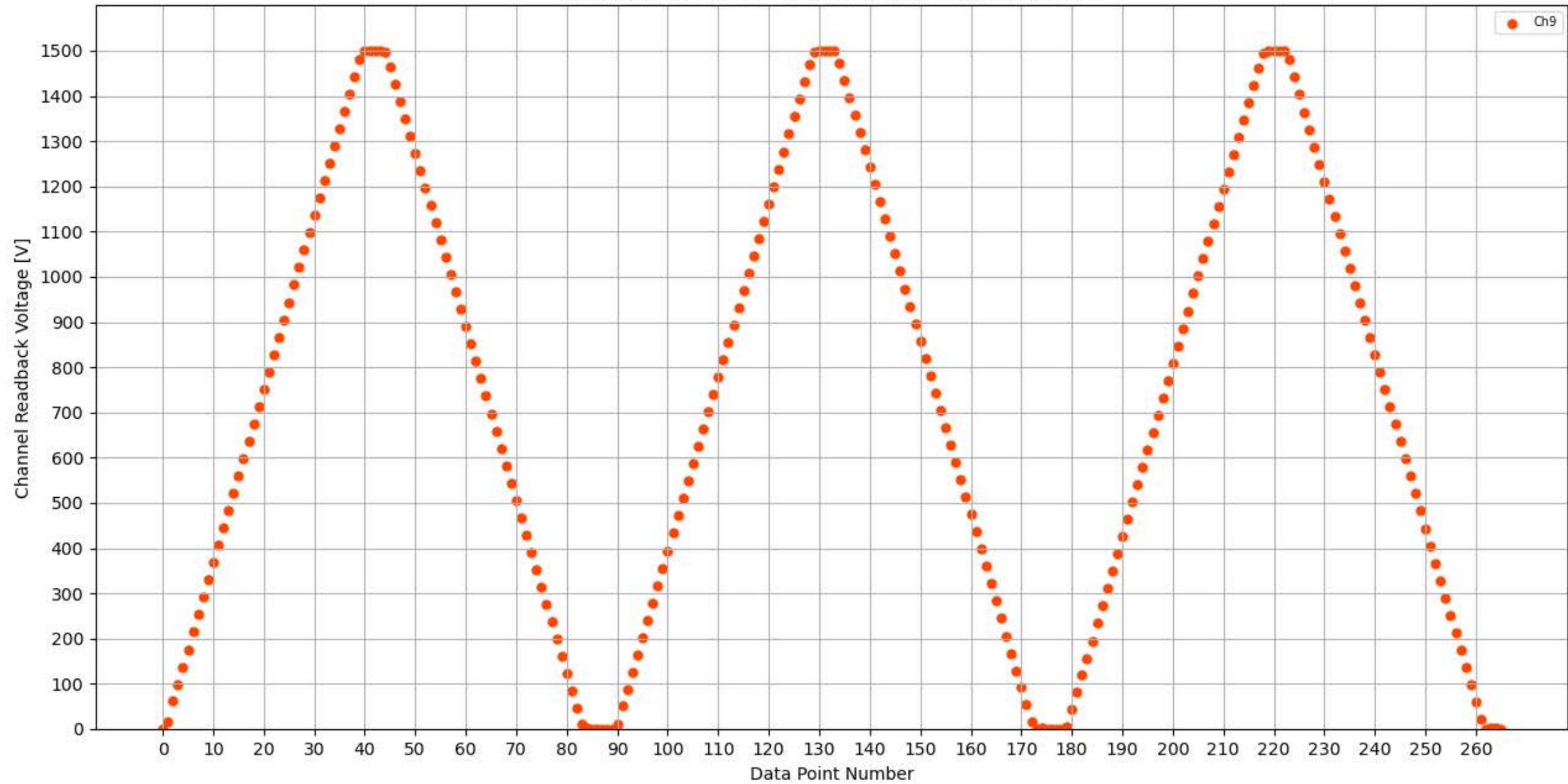
Voltage Ramp Test (Python) Bd #326, Slot #6, Ch #9
