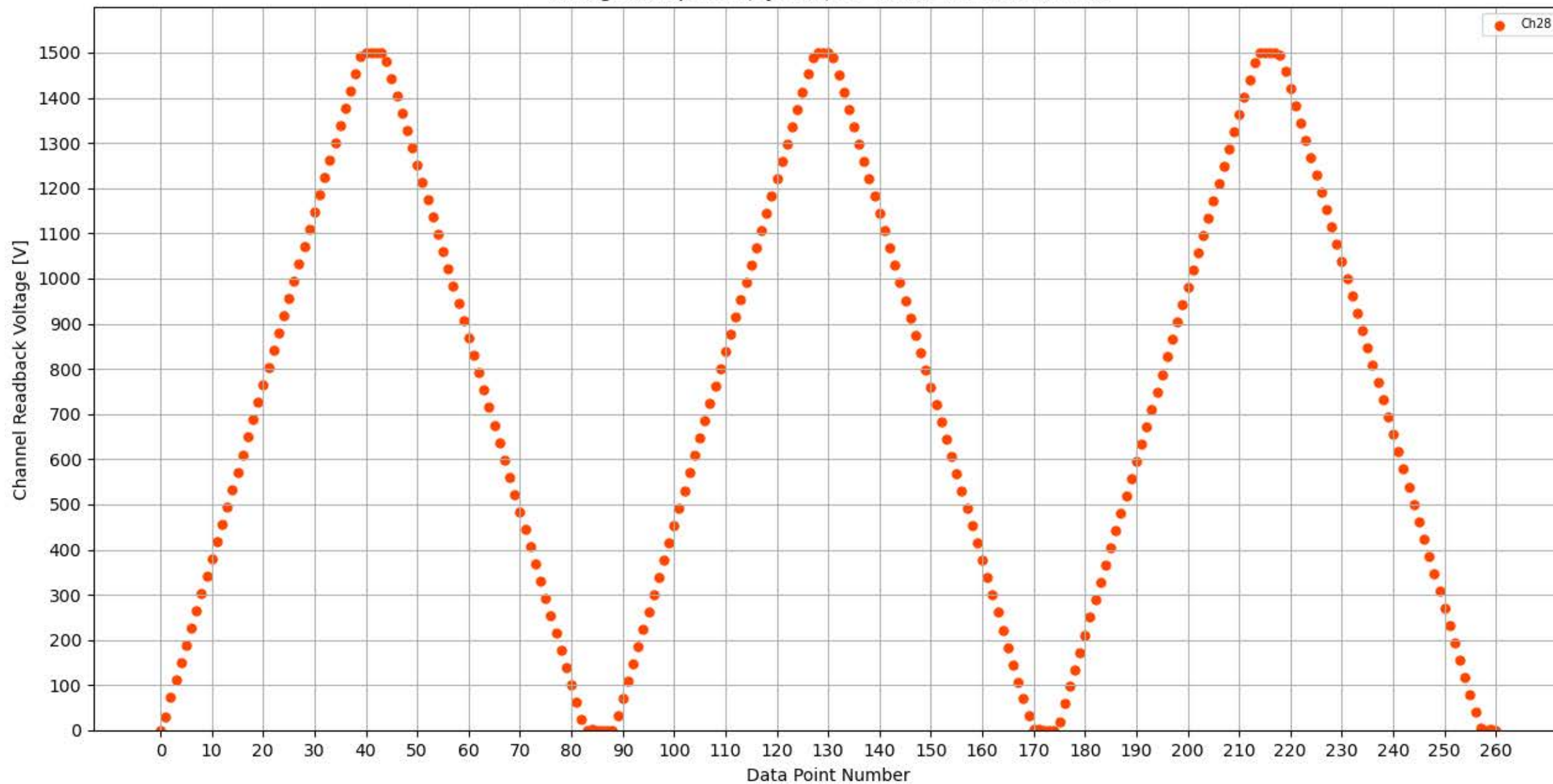
Voltage Ramp Test (Python) Bd #326, Slot #6, Ch #28
