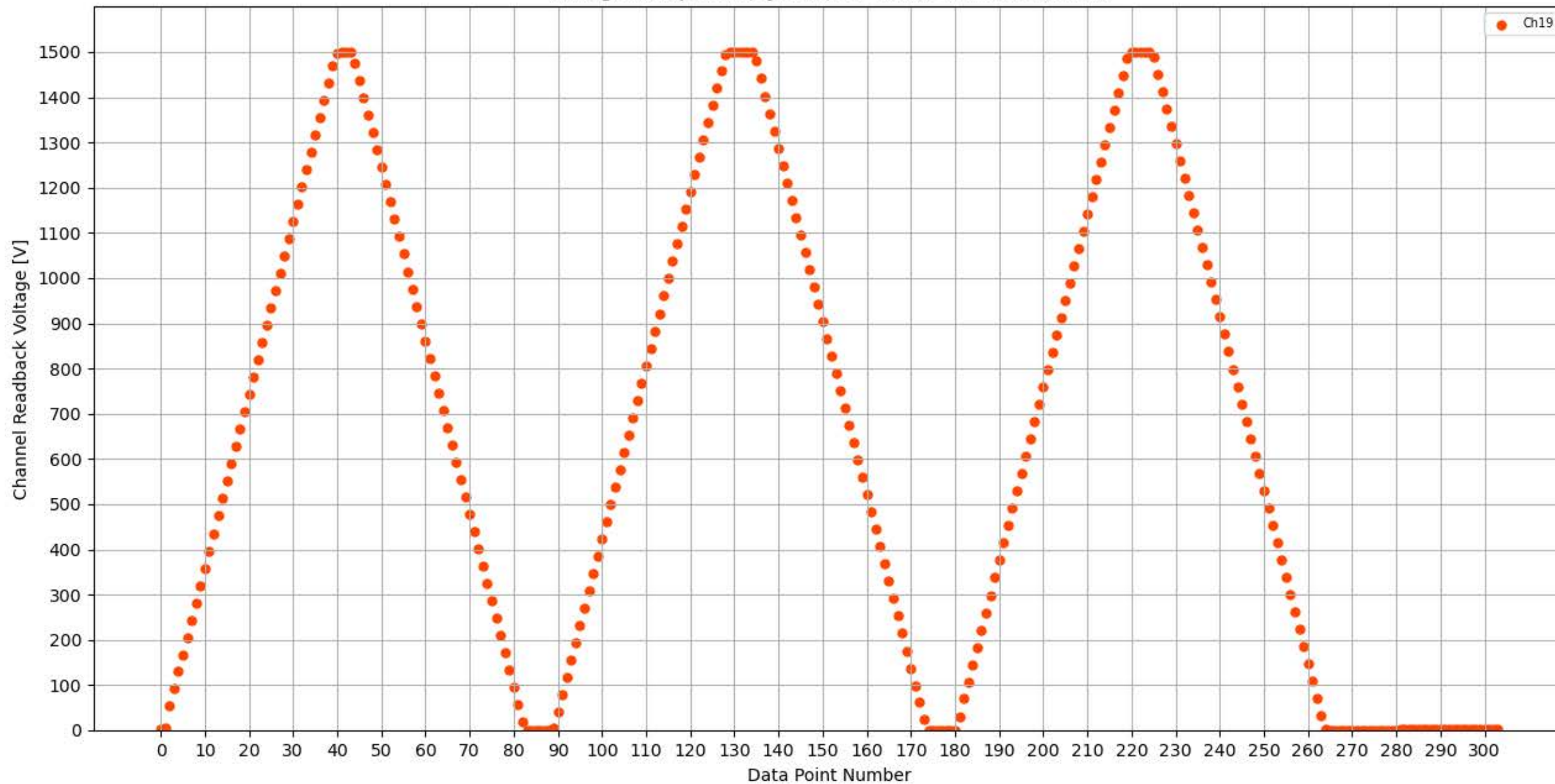
Voltage Ramp Test (Python) Bd #326, Slot #6, Ch #19
