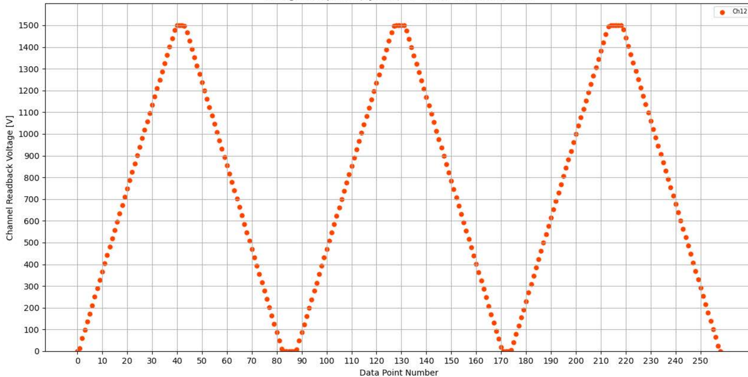
Voltage Ramp Test (Python) Bd #326, Slot #6, Ch #12
