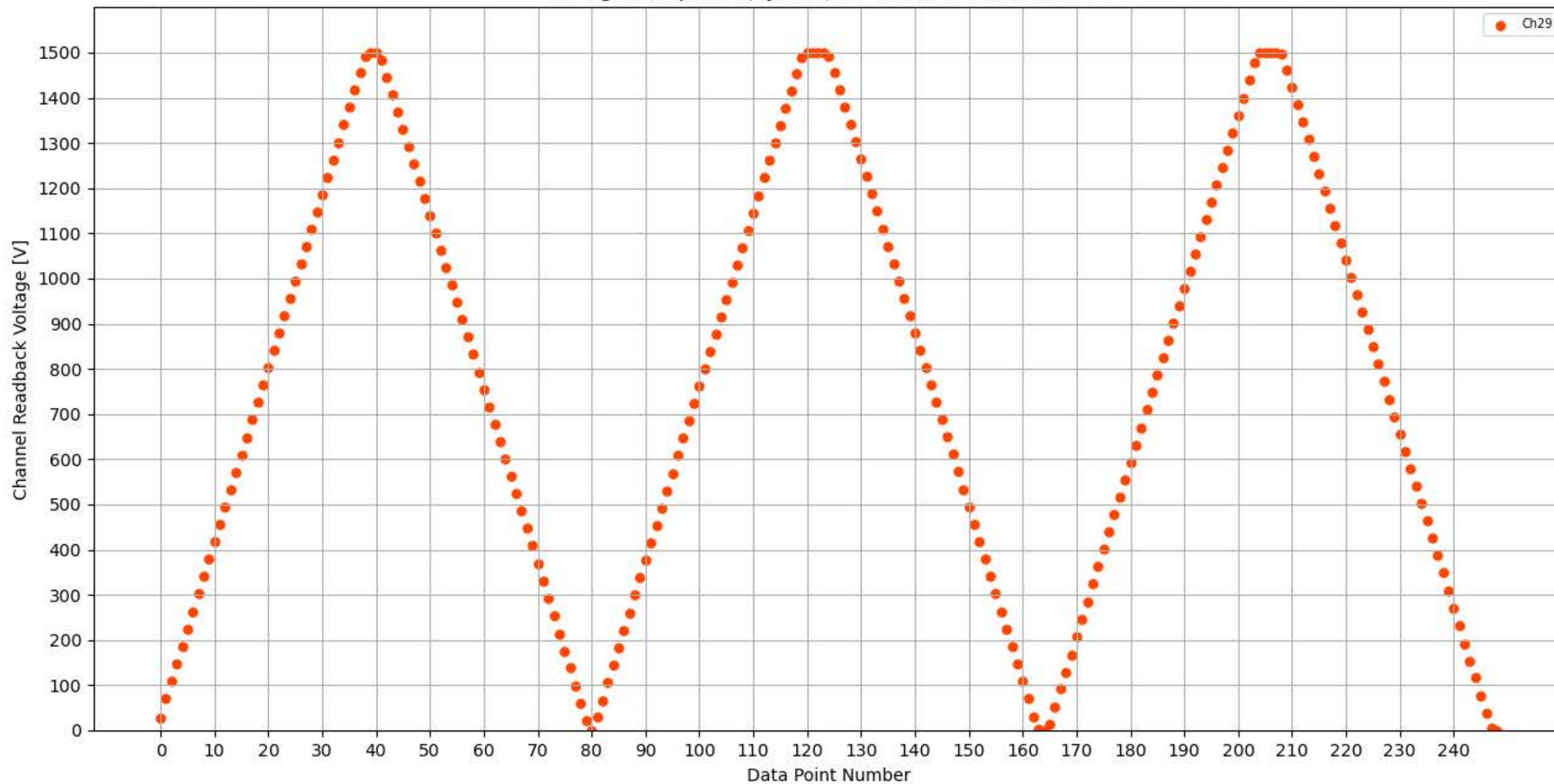
Voltage Ramp Test (Python) Bd #326, Slot #6, Ch #29
