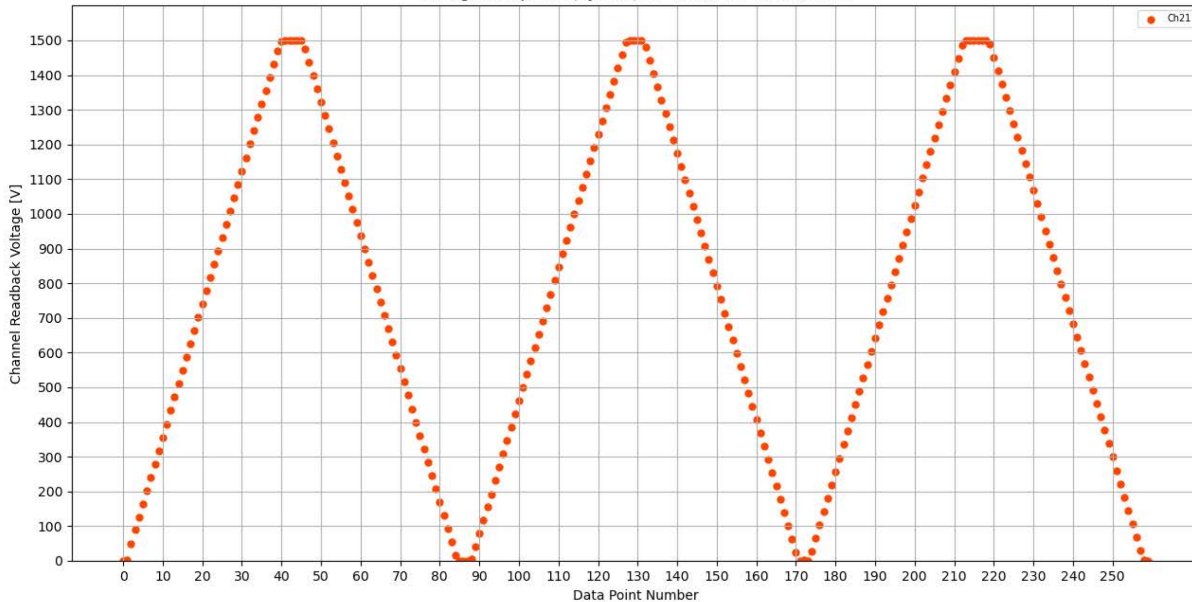
Voltage Ramp Test (Python) Bd #326, Slot #6, Ch #21
