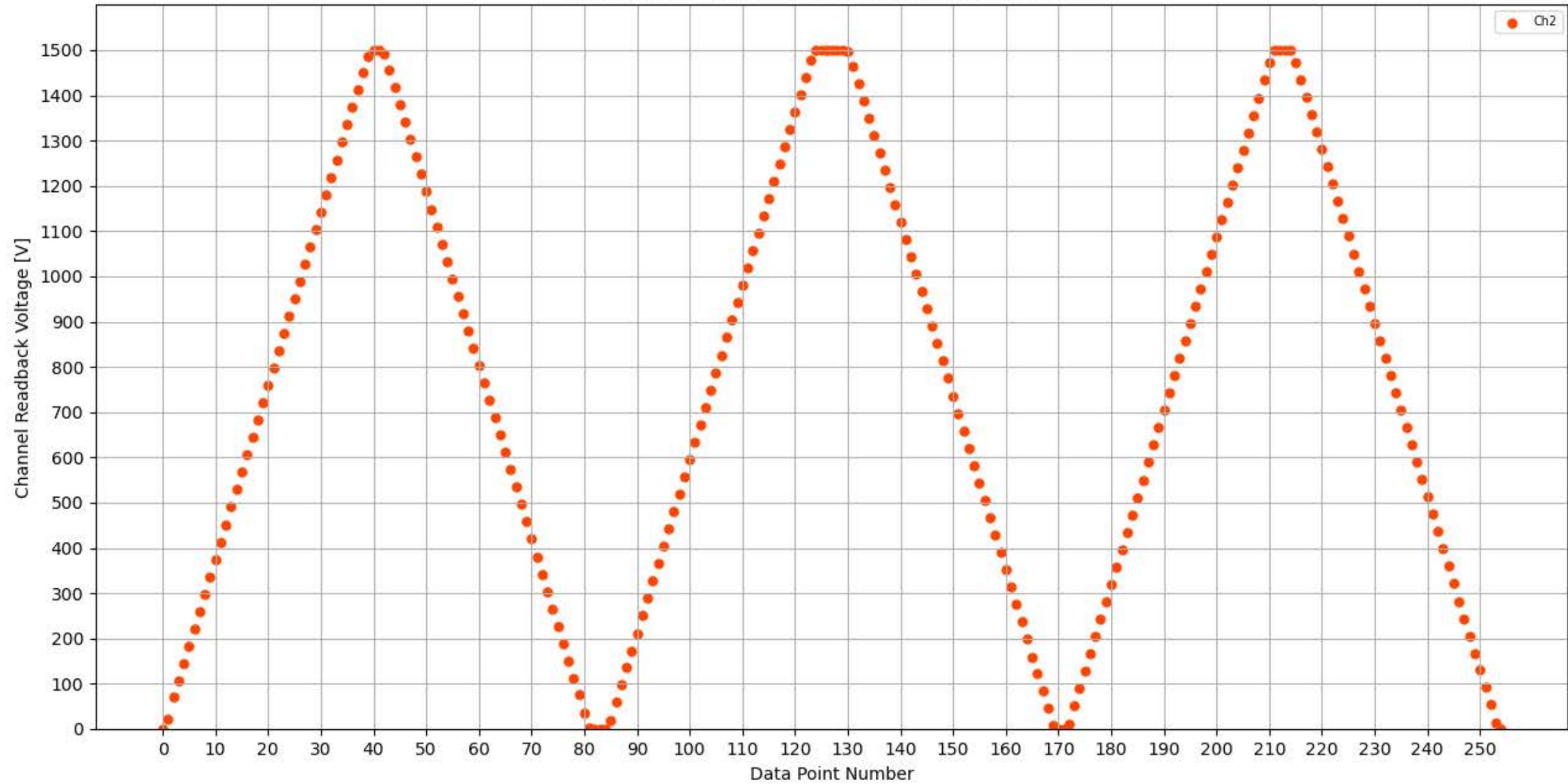
Voltage Ramp Test (Python) Bd #326, Slot #6, Ch #2
