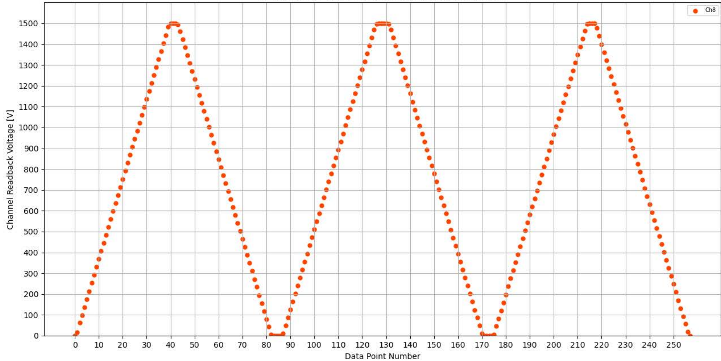
Voltage Ramp Test (Python) Bd #326, Slot #6, Ch #8
