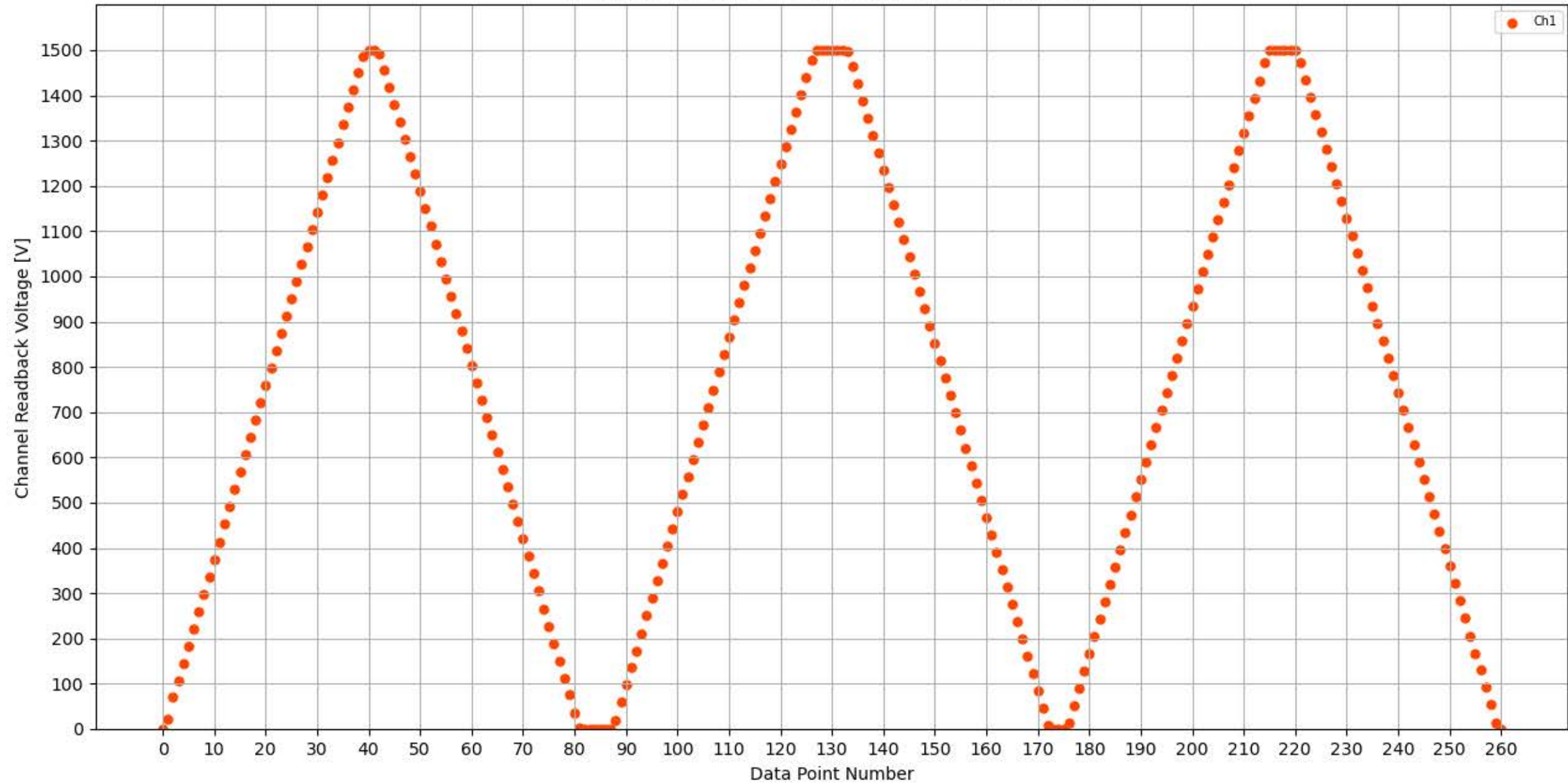
Voltage Ramp Test (Python) Bd #326, Slot #6, Ch #1
