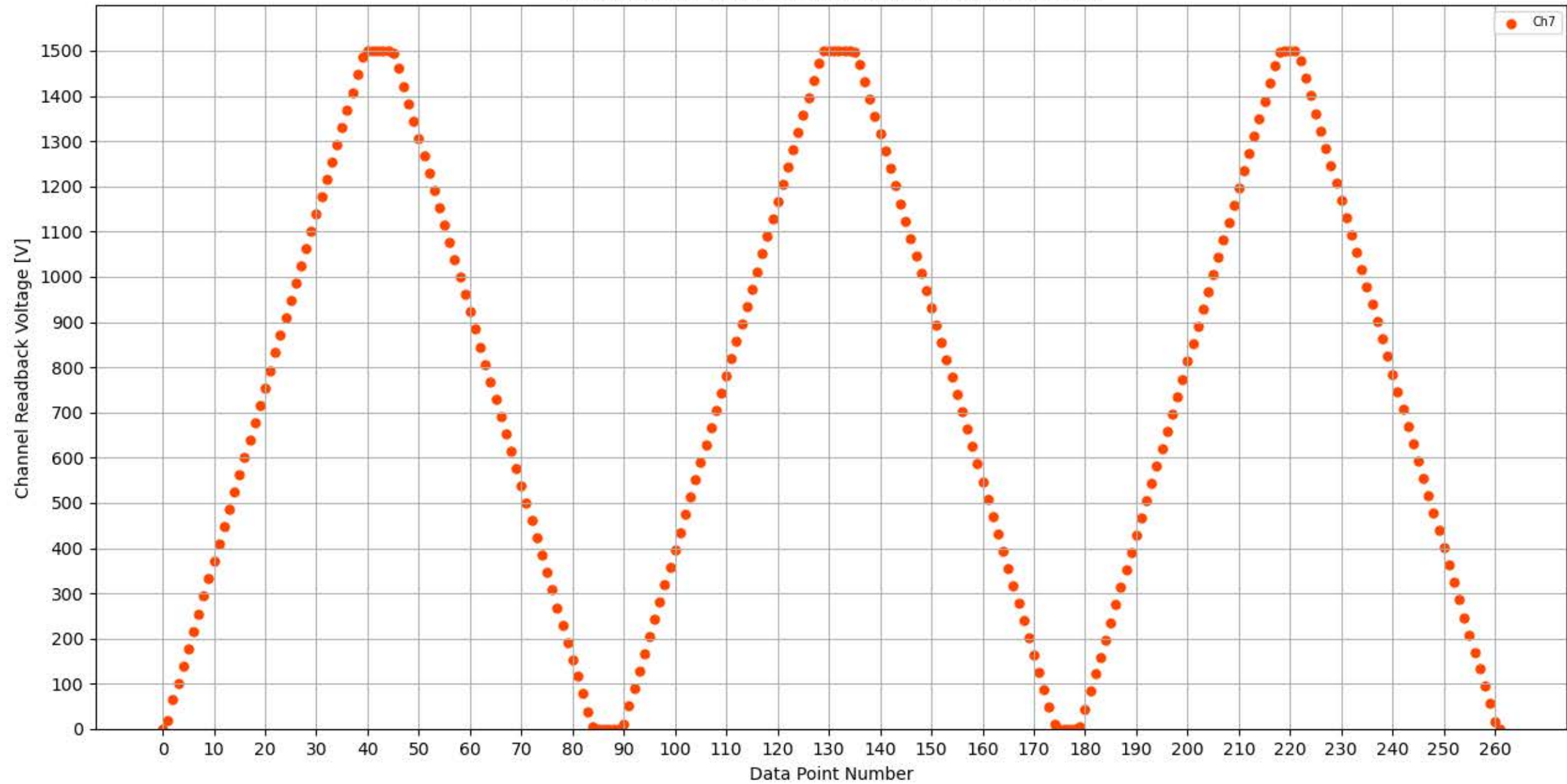
Voltage Ramp Test (Python) Bd #326, Slot #6, Ch #7
