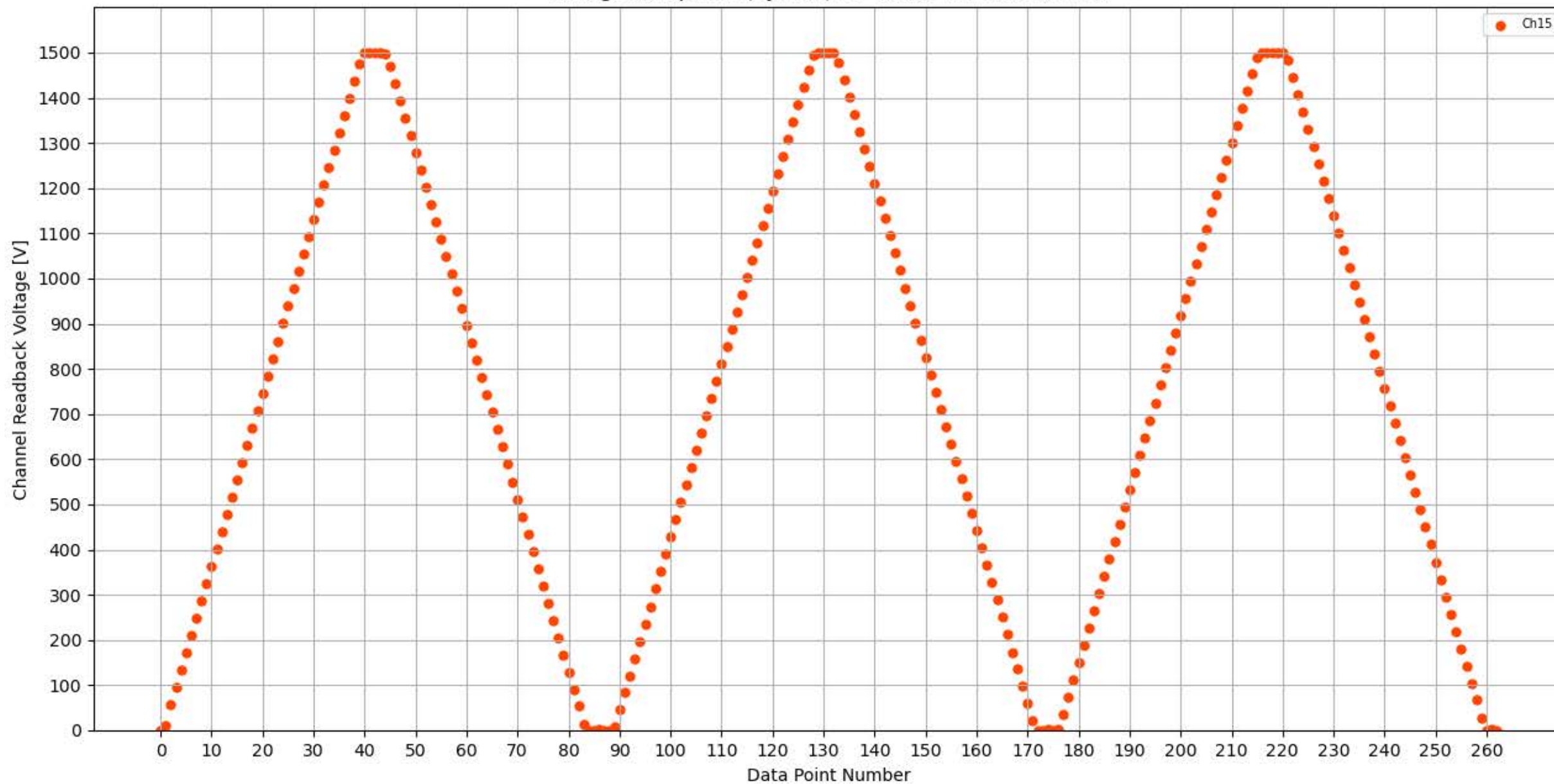
Voltage Ramp Test (Python) Bd #326, Slot #6, Ch #15
