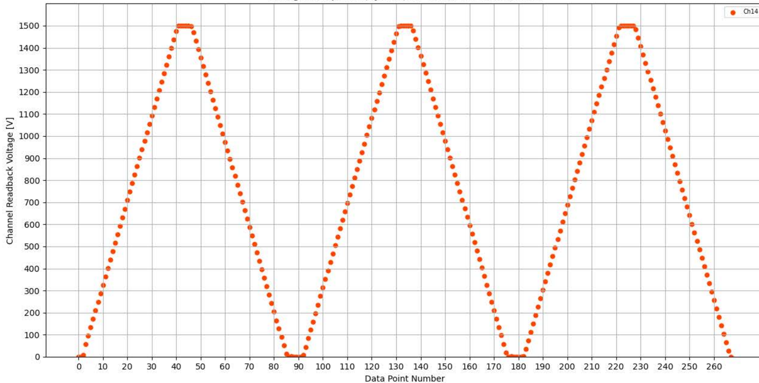
Voltage Ramp Test (Python) Bd #326, Slot #6, Ch #14
