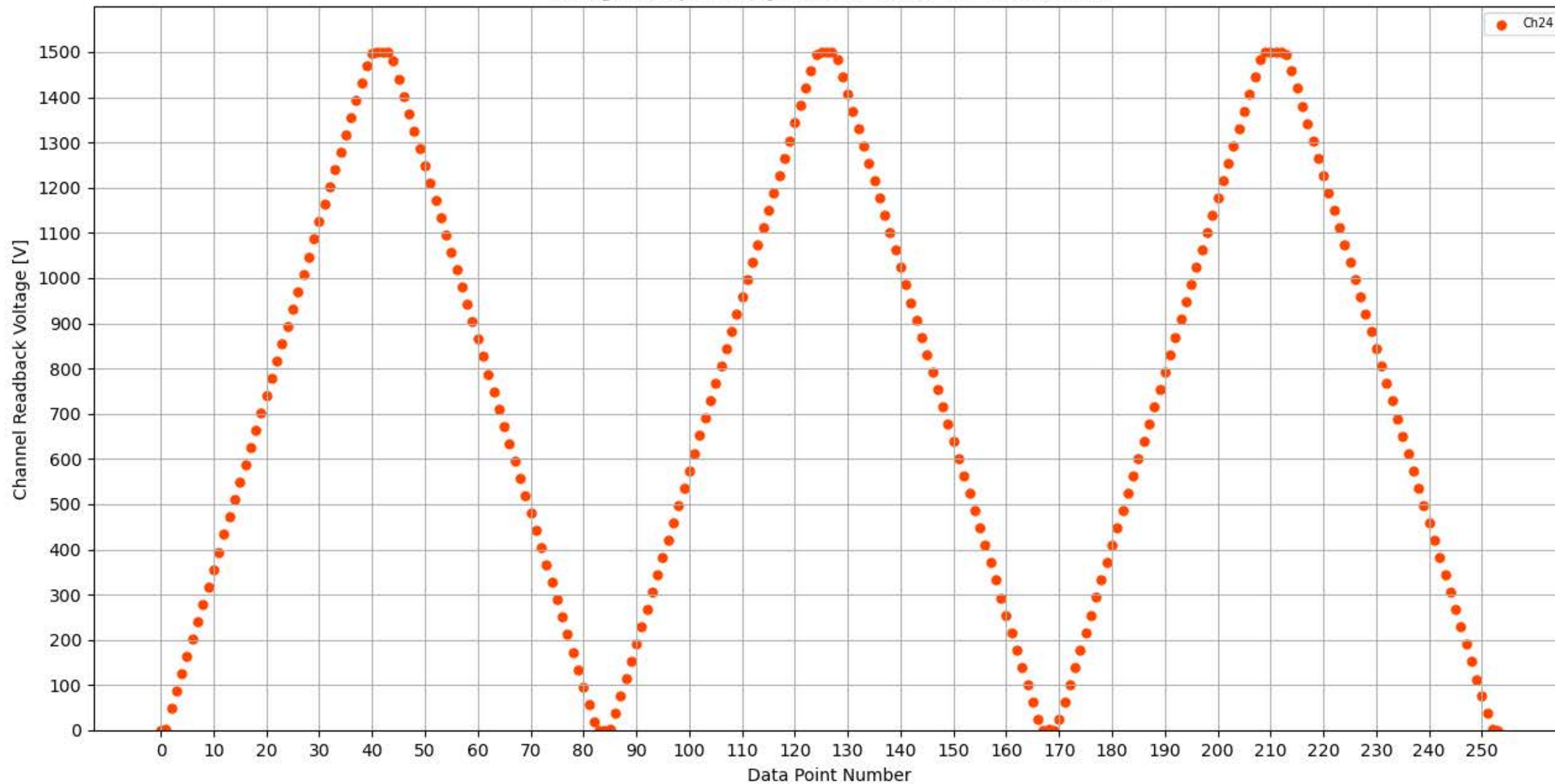
Voltage Ramp Test (Python) Bd #326, Slot #6, Ch #24
