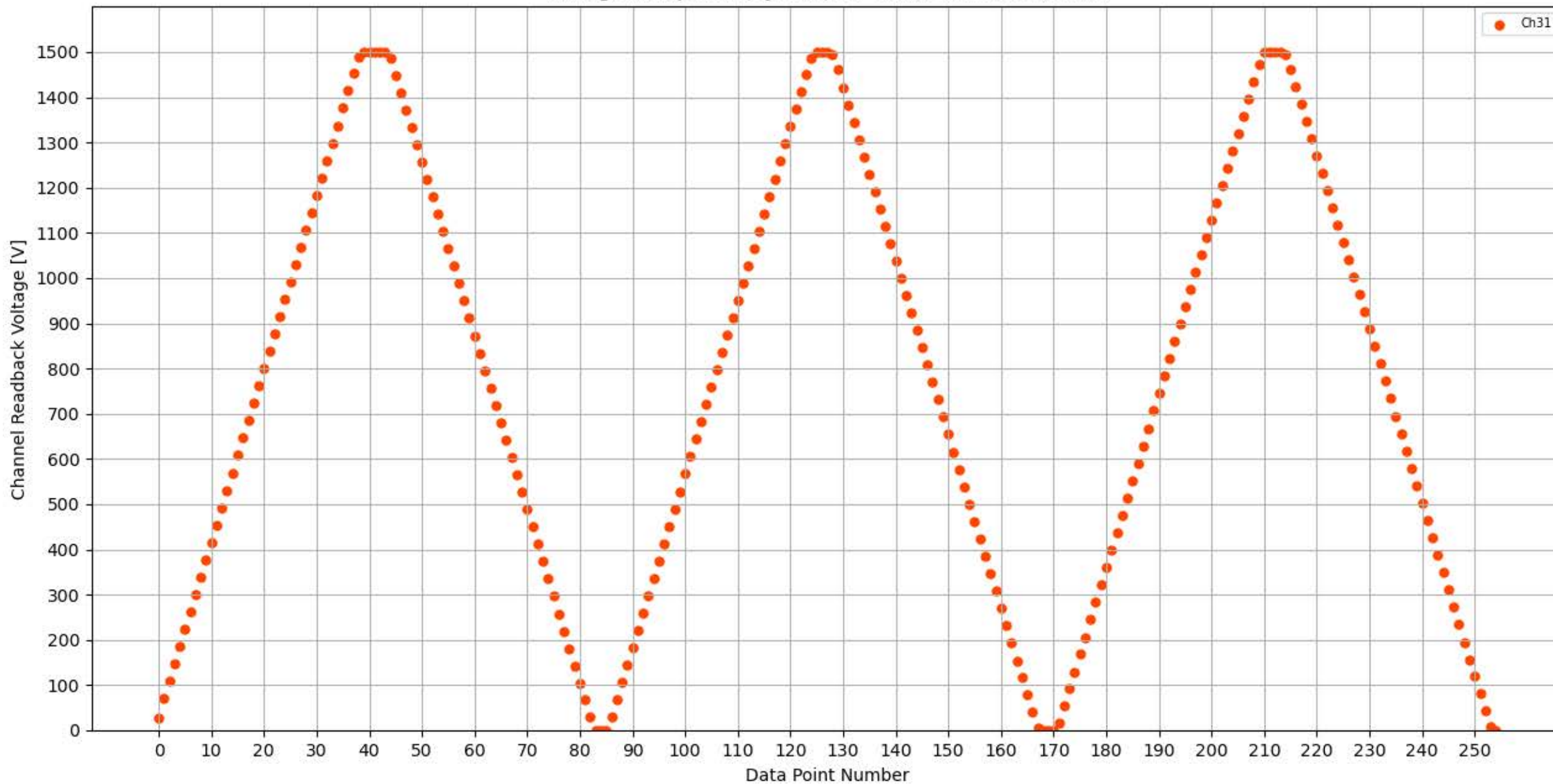
Voltage Ramp Test (Python) Bd #326, Slot #6, Ch #31
