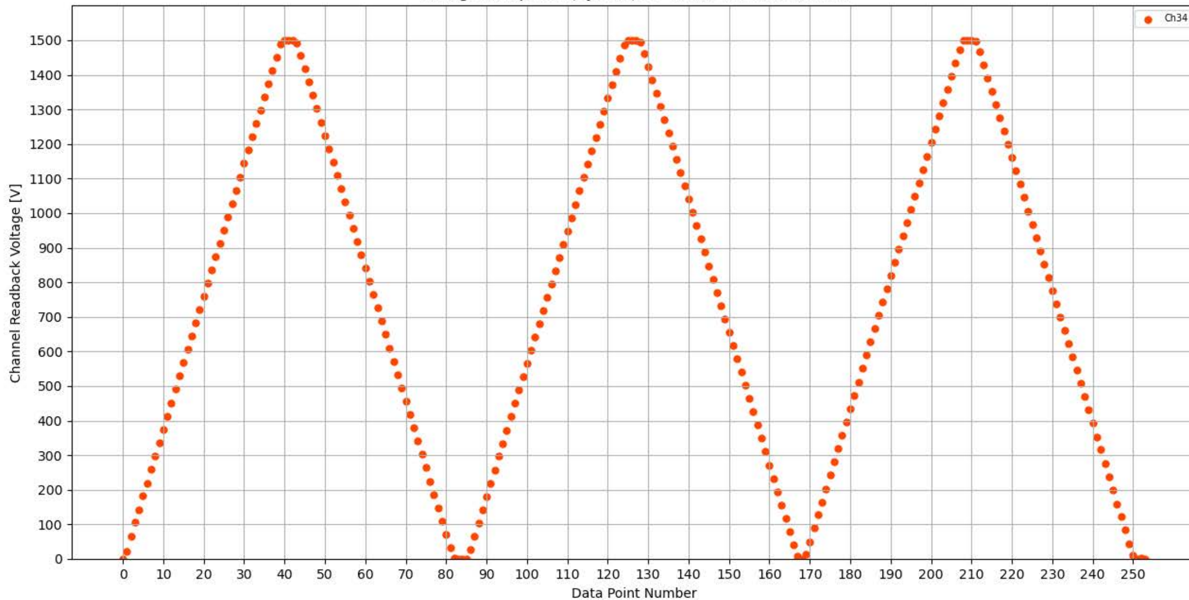
Voltage Ramp Test (Python) Bd #326, Slot #6, Ch #34
