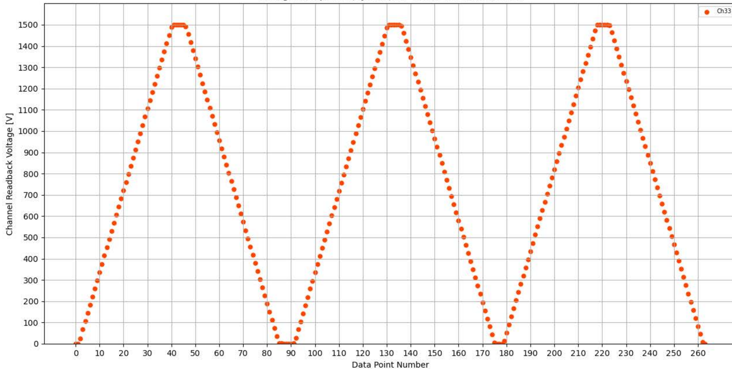
Voltage Ramp Test (Python) Bd #326, Slot #6, Ch #33
