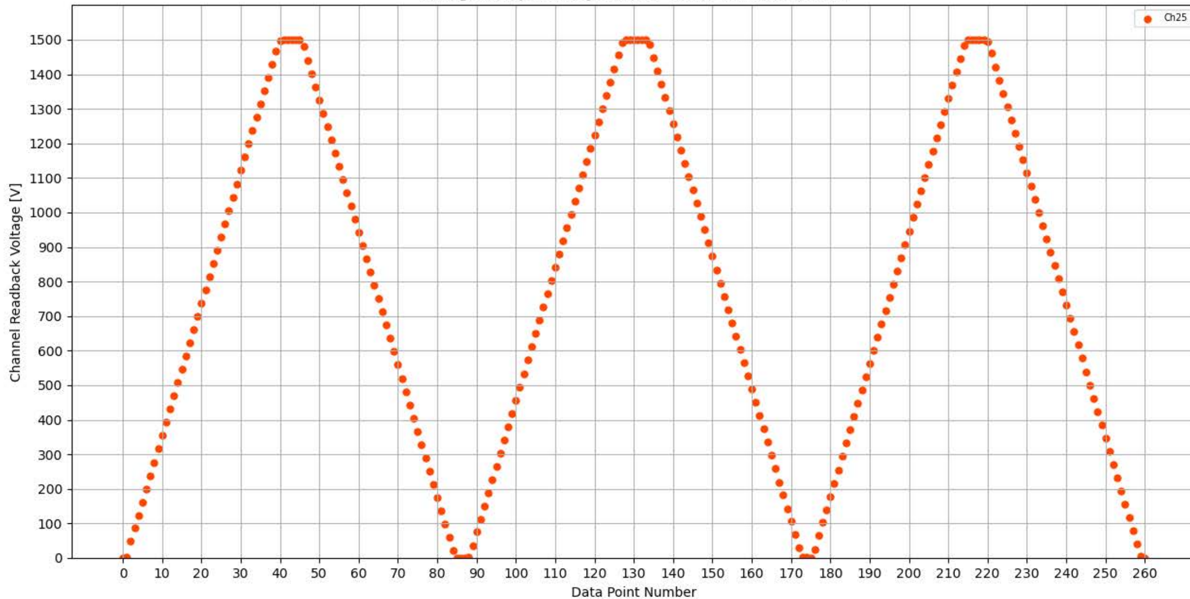
Voltage Ramp Test (Python) Bd #326, Slot #6, Ch #25
