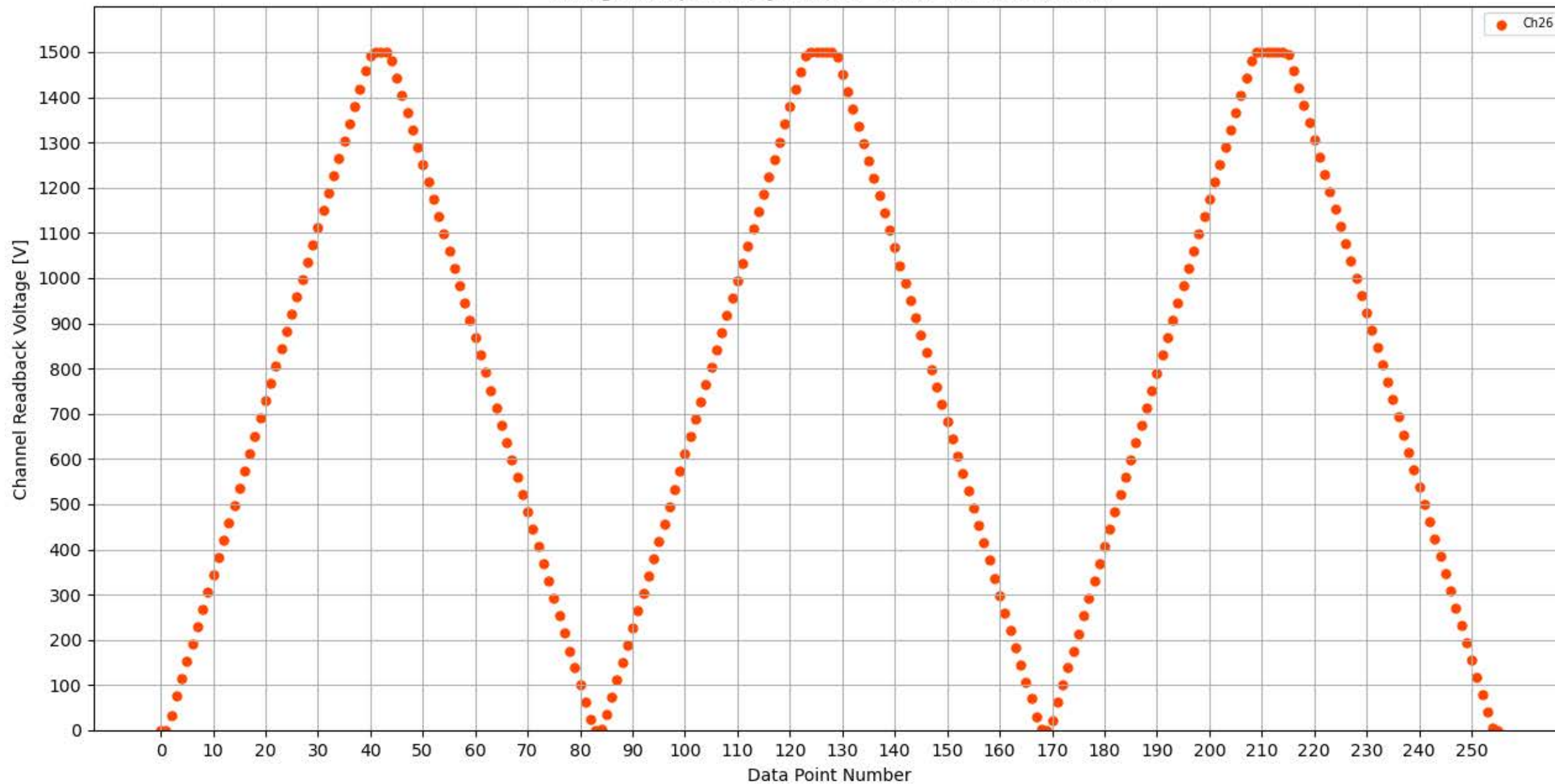
Voltage Ramp Test (Python) Bd #326, Slot #6, Ch #26
