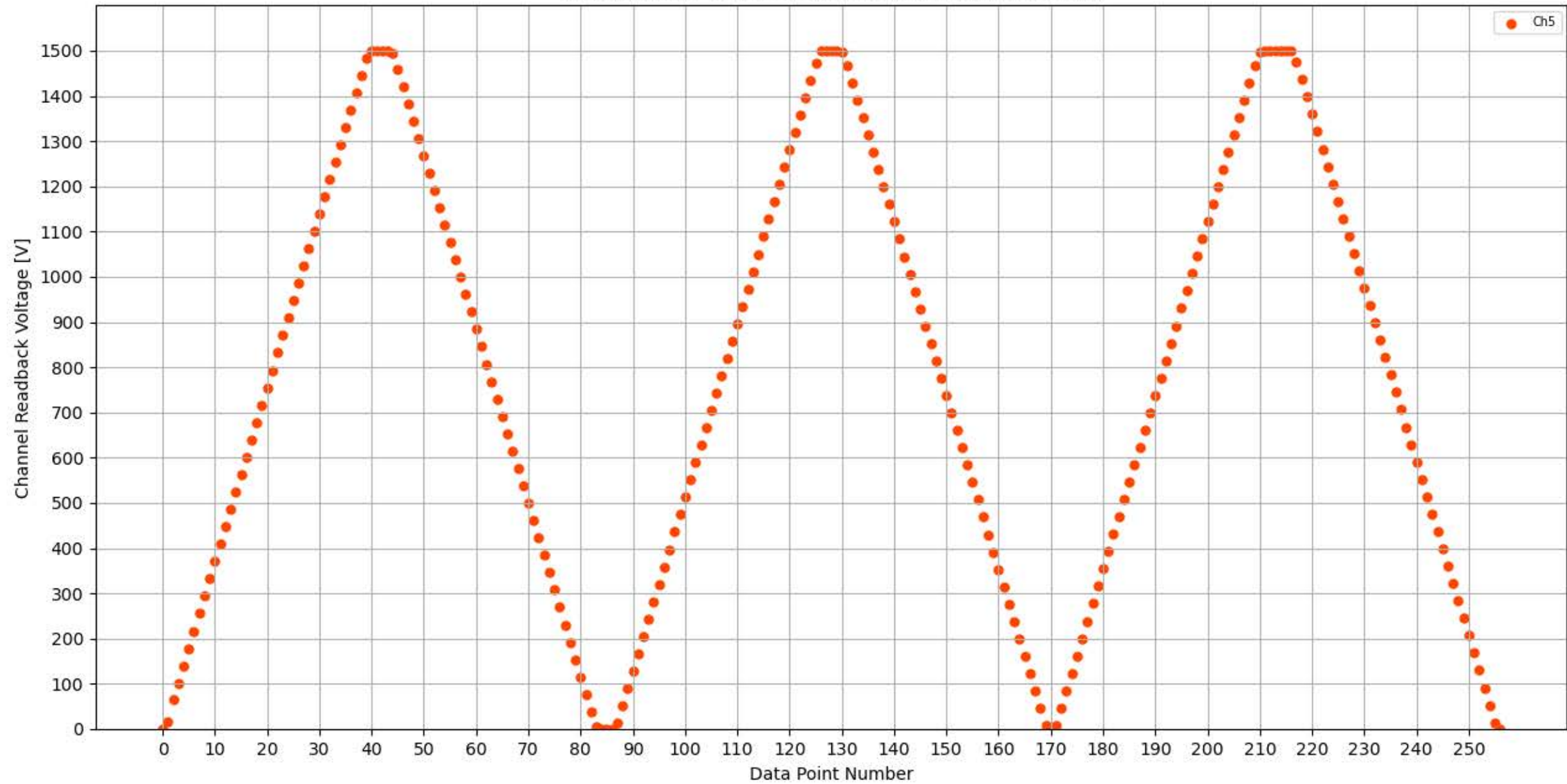
Voltage Ramp Test (Python) Bd #326, Slot #6, Ch #5
