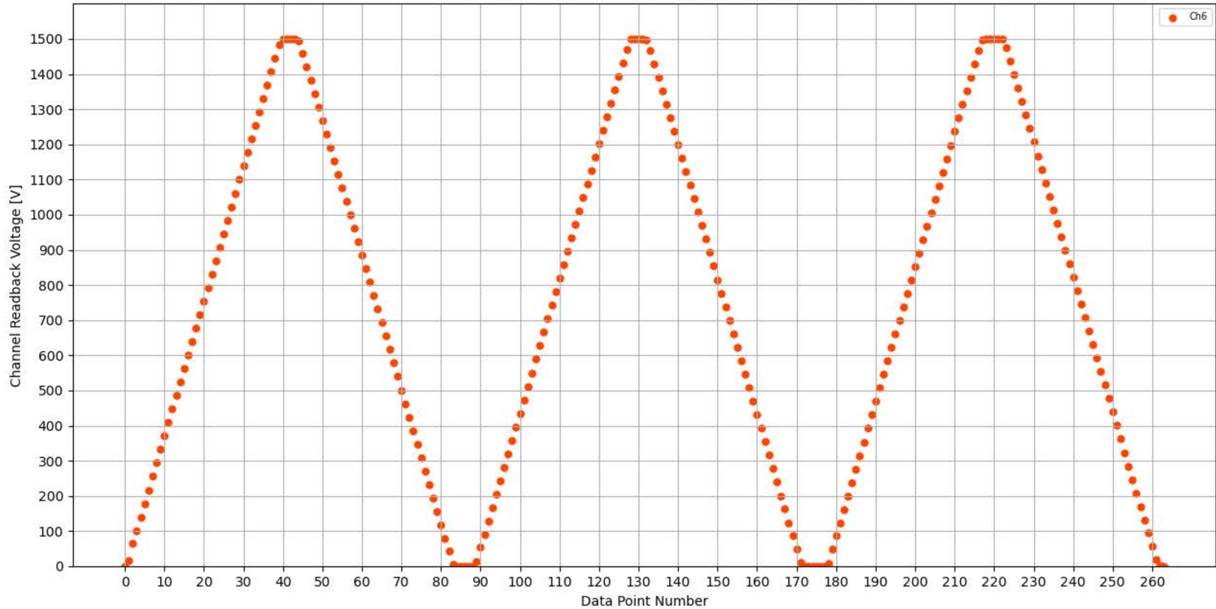
Voltage Ramp Test (Python) Bd #326, Slot #6, Ch #6
