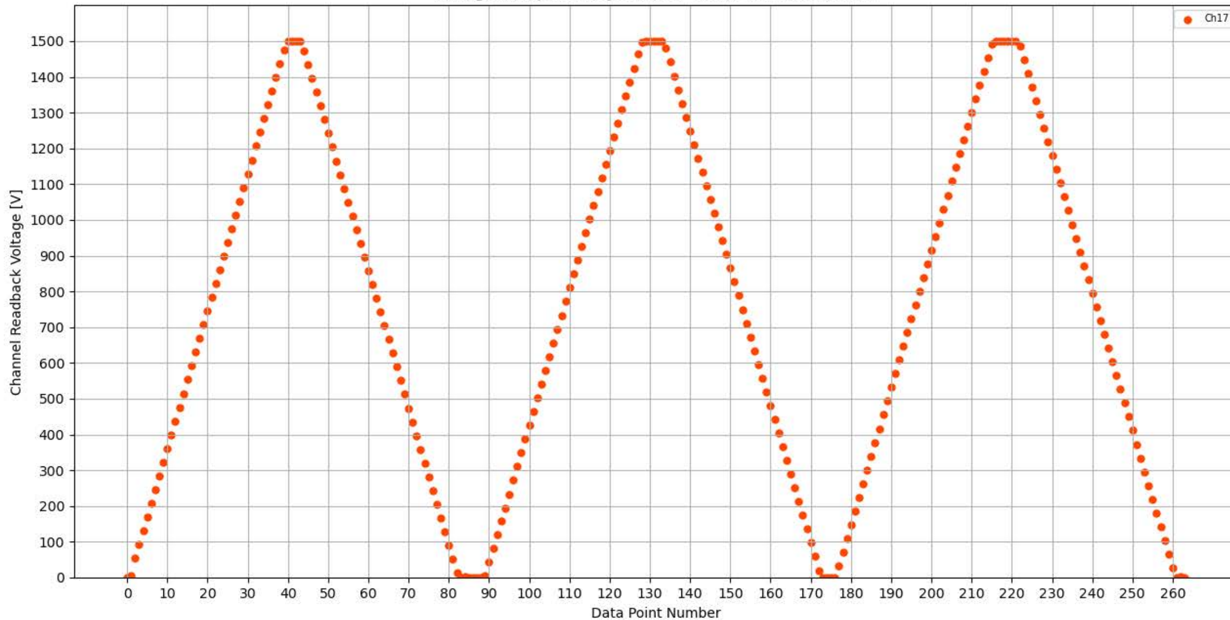
Voltage Ramp Test (Python) Bd #326, Slot #6, Ch #17
