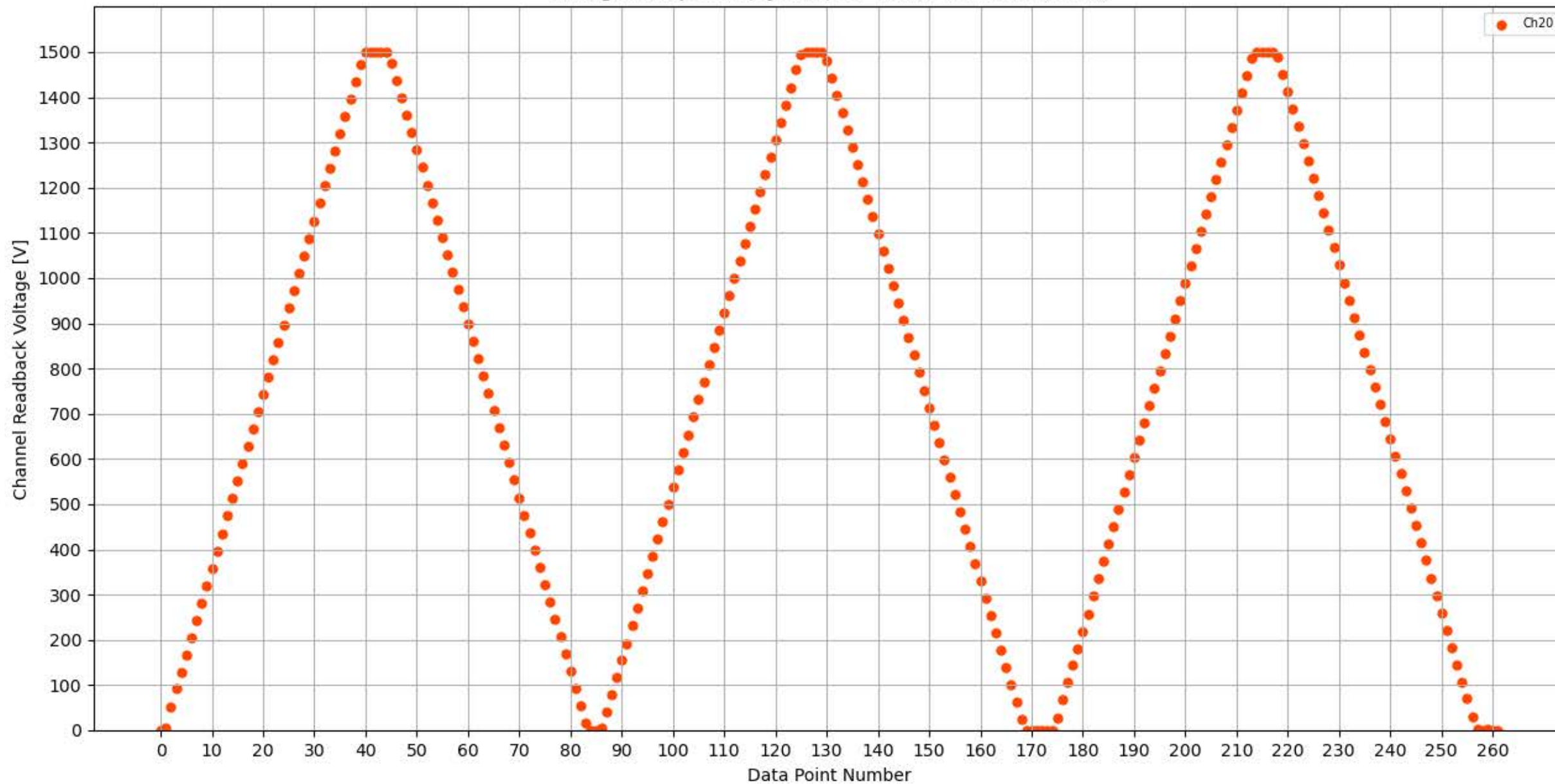
Voltage Ramp Test (Python) Bd #326, Slot #6, Ch #20
