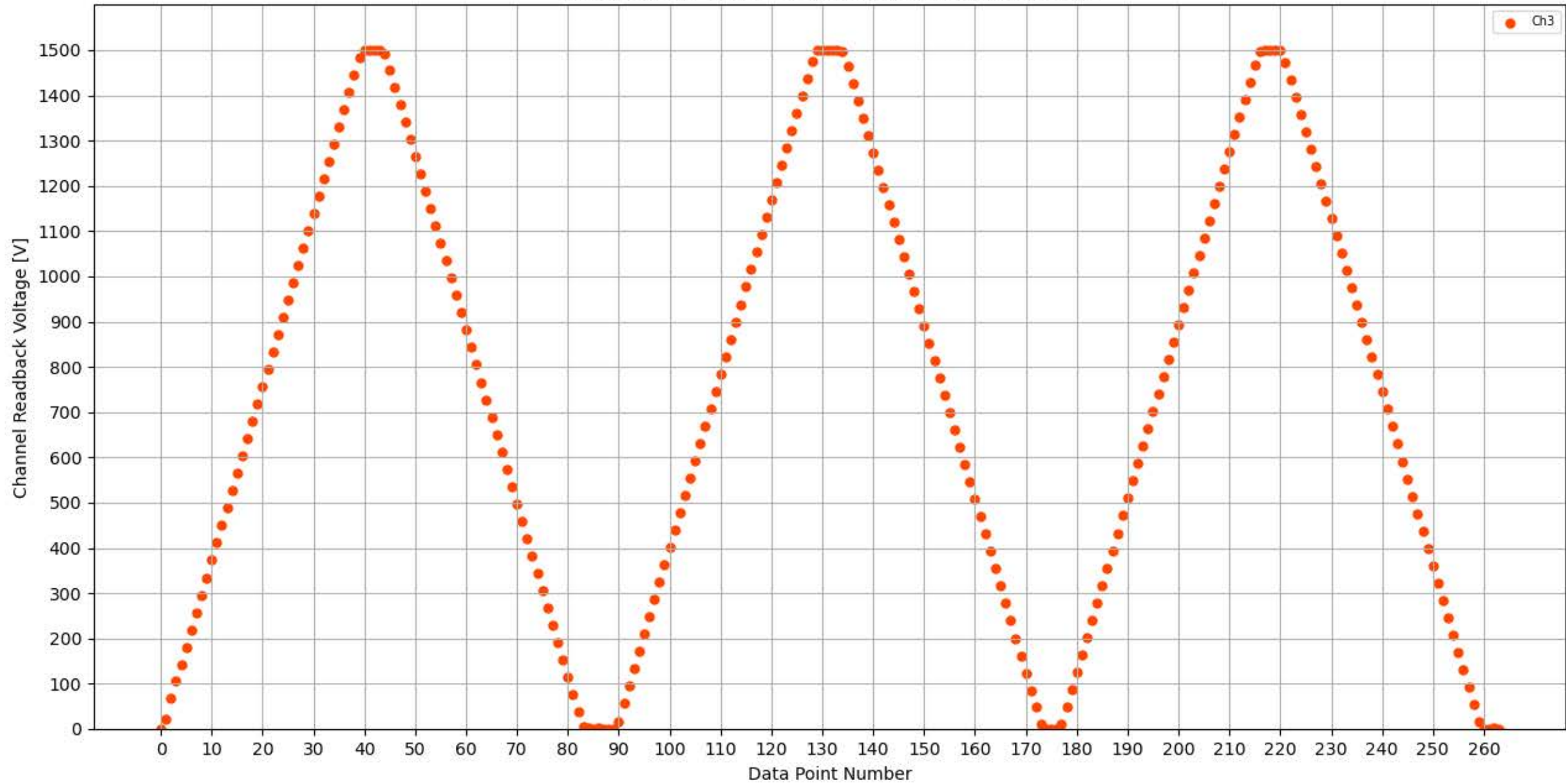
Voltage Ramp Test (Python) Bd #326, Slot #6, Ch #3
